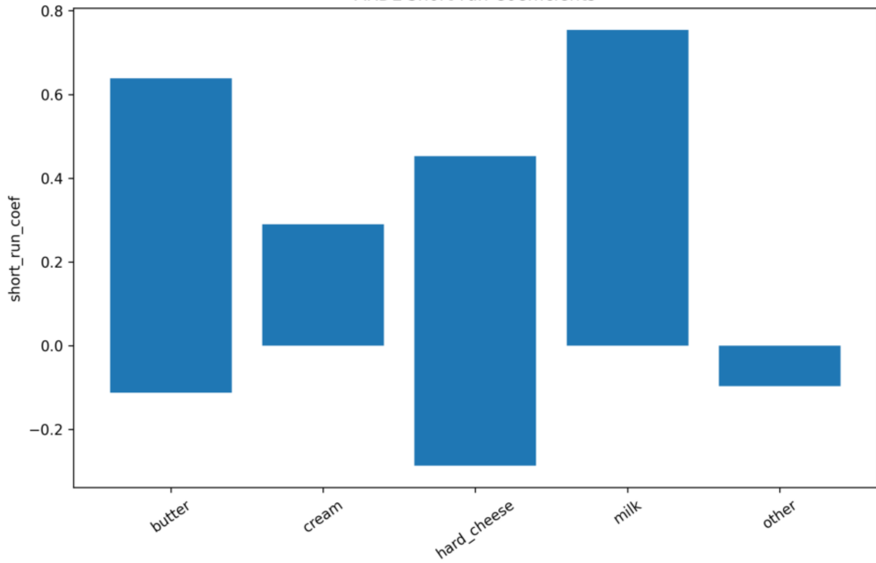
ARDL Short-run Coefficients
